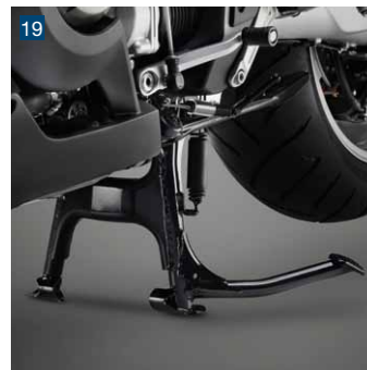
19 Mainstand A necessity for more secure parking on variable ground surfaces, a Mainstand also facilitates cleaning and rear wheel maintenance.
